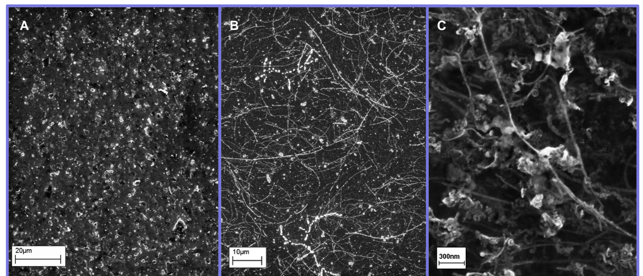
Fig 3: SEM images of field emitters fabricated using CNT types A, B & C
