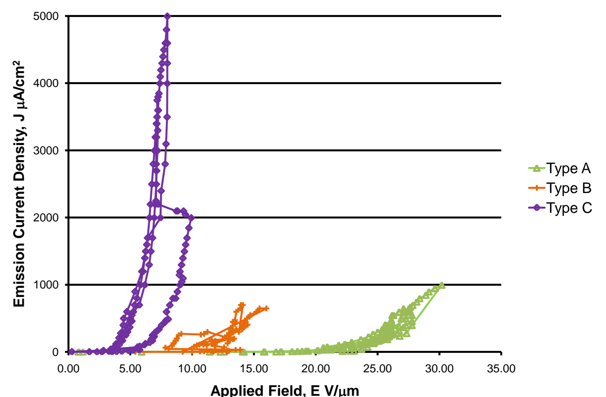
Fig 4: Plot of field emission performance of printed emitters
