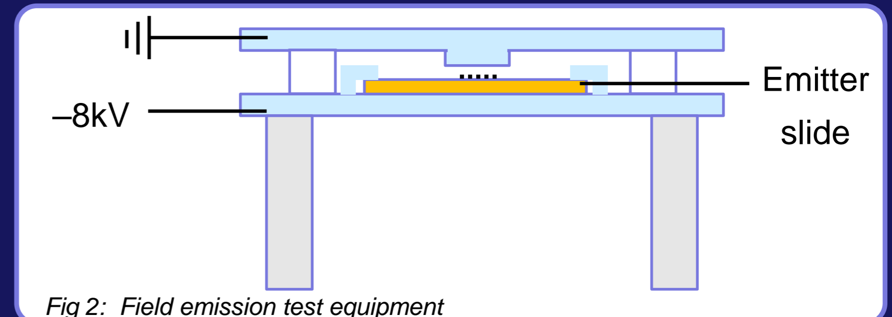
Fig 2: Field emission test equipment
