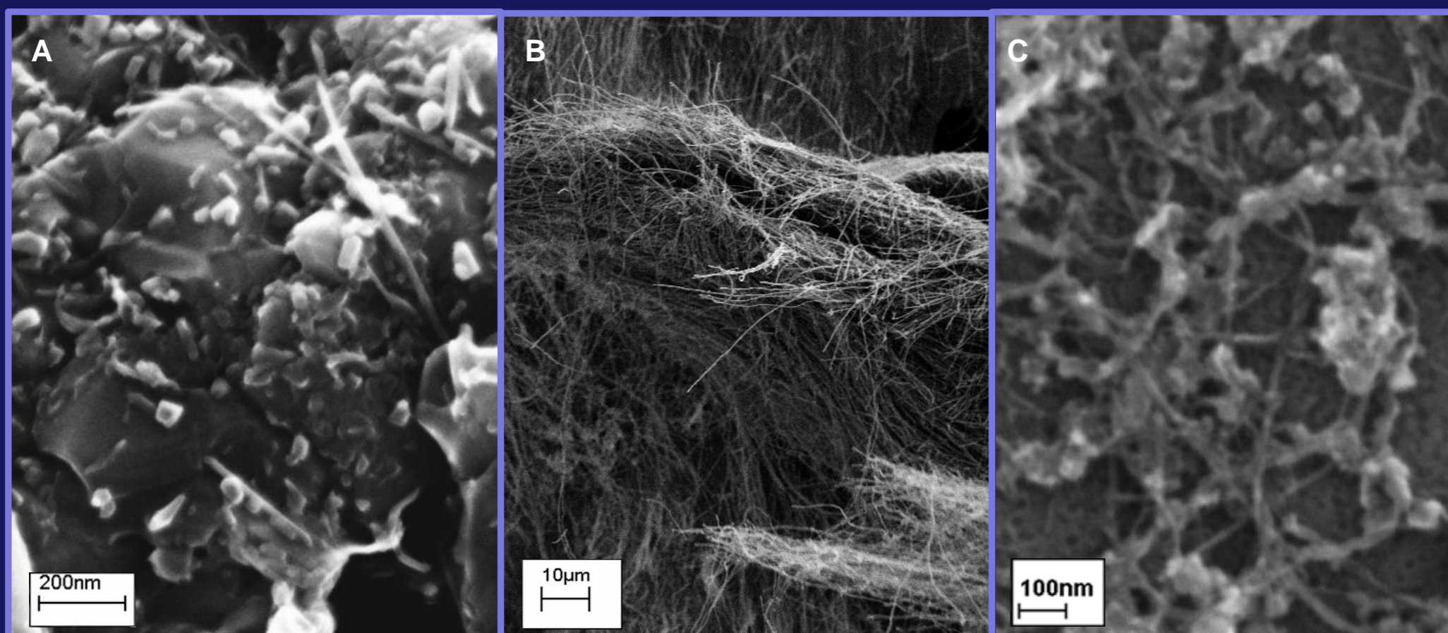
Fig 1: Scanning electron microscope (SEM) images of MWCNT types A, B & C
